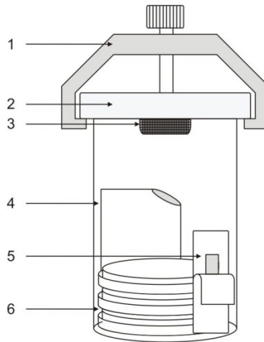
Fig. 22. The anaerobic jar. (1) clamp (2) cover (3) palladium catalyst (4) H 2 +CO 2 generator (5) redox indicator (6) culture plates.
