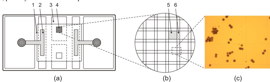
Fig. 11. Bürker-chamber. (a) Parts of the chamber 1. cover glass 2. clamp 3. counting chamber (drop the spore suspension here) 4. facet with grid (b) Enlarged grid 5. big square of 1/25 \text{ mm}^2 area 6. rectangle of 1/100 \text{ mm}^2 area. (c) Micrograph of spores from Aspergillus niger in a Bürker chamber.
